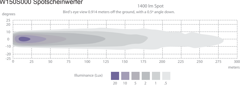
W150S000 Spotscheinwerfer
